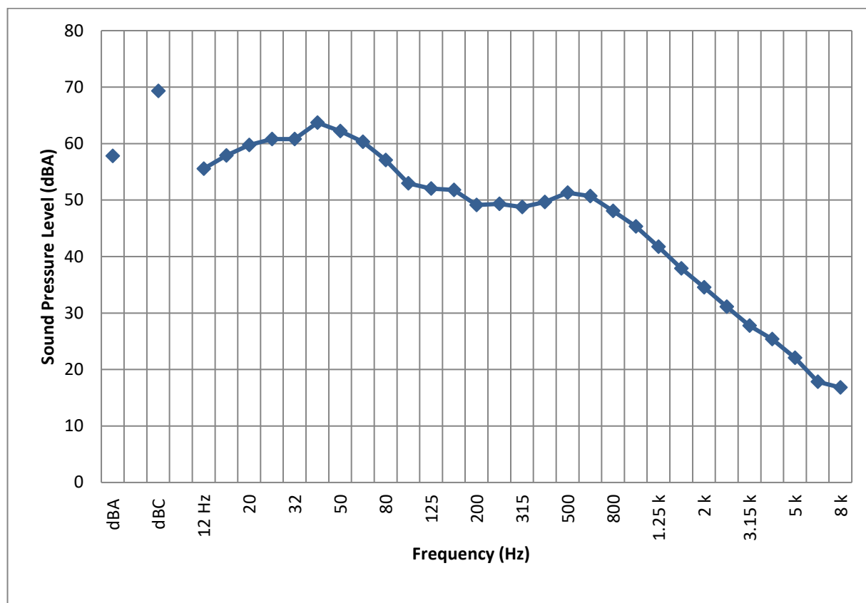
Figure 9. Noise Monitor (44 Andrew Crescent) – 24-Hour 1/3 Octave Band L_{eq} Sound Levels
