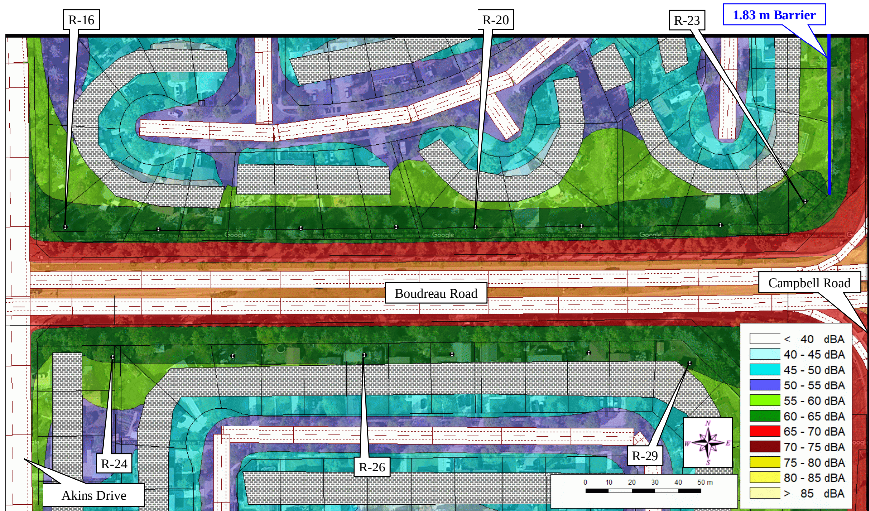
Figure 17. Future Case L_{eq24} Noise Levels (East)
