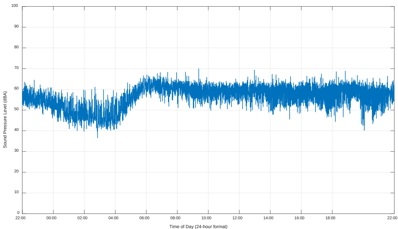
Figure 12. Noise Monitor (52 Andrew Crescent) – 15-Second L_{eq24} Sound Levels
