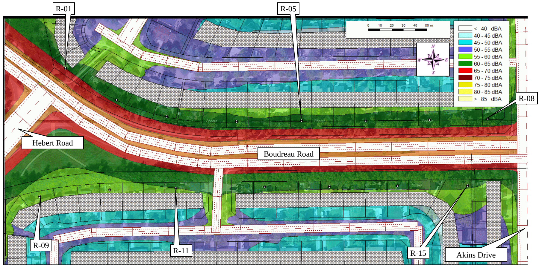
Figure 16. Future Case L_{eq24} Noise Levels (West)
