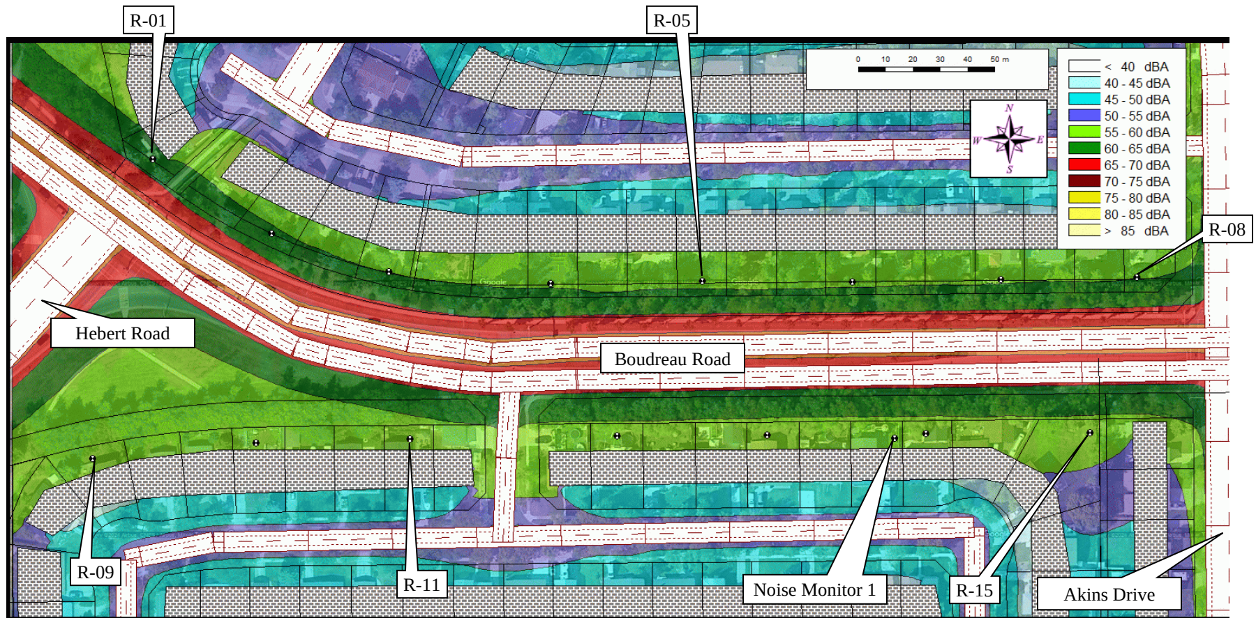
Figure 14. Baseline Case L_{eq24} Noise Levels (West)
