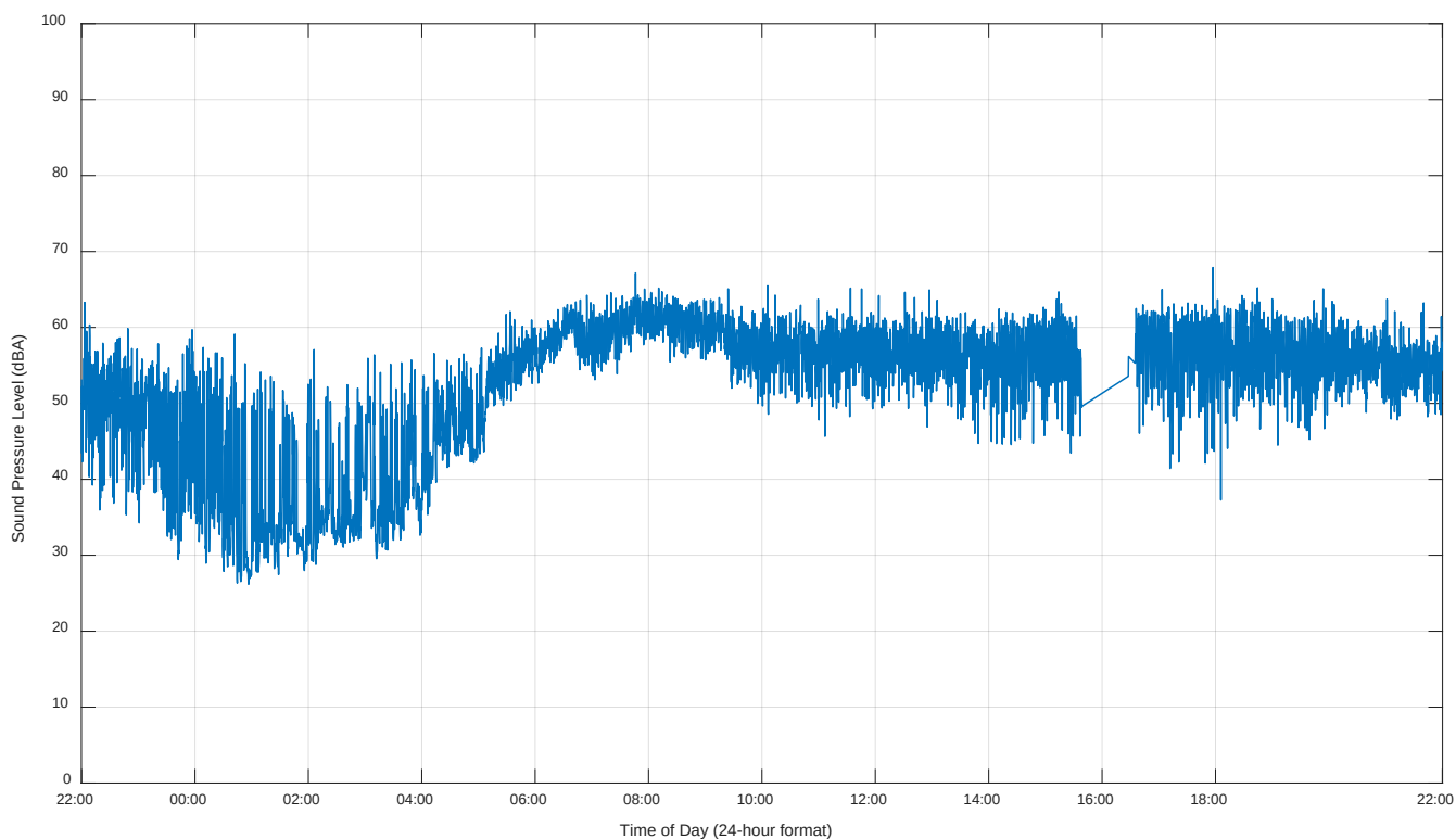
Figure 6. Noise Monitor (60 Aspen Crescent) – 15-Second L_{eq24} Sound Levels
