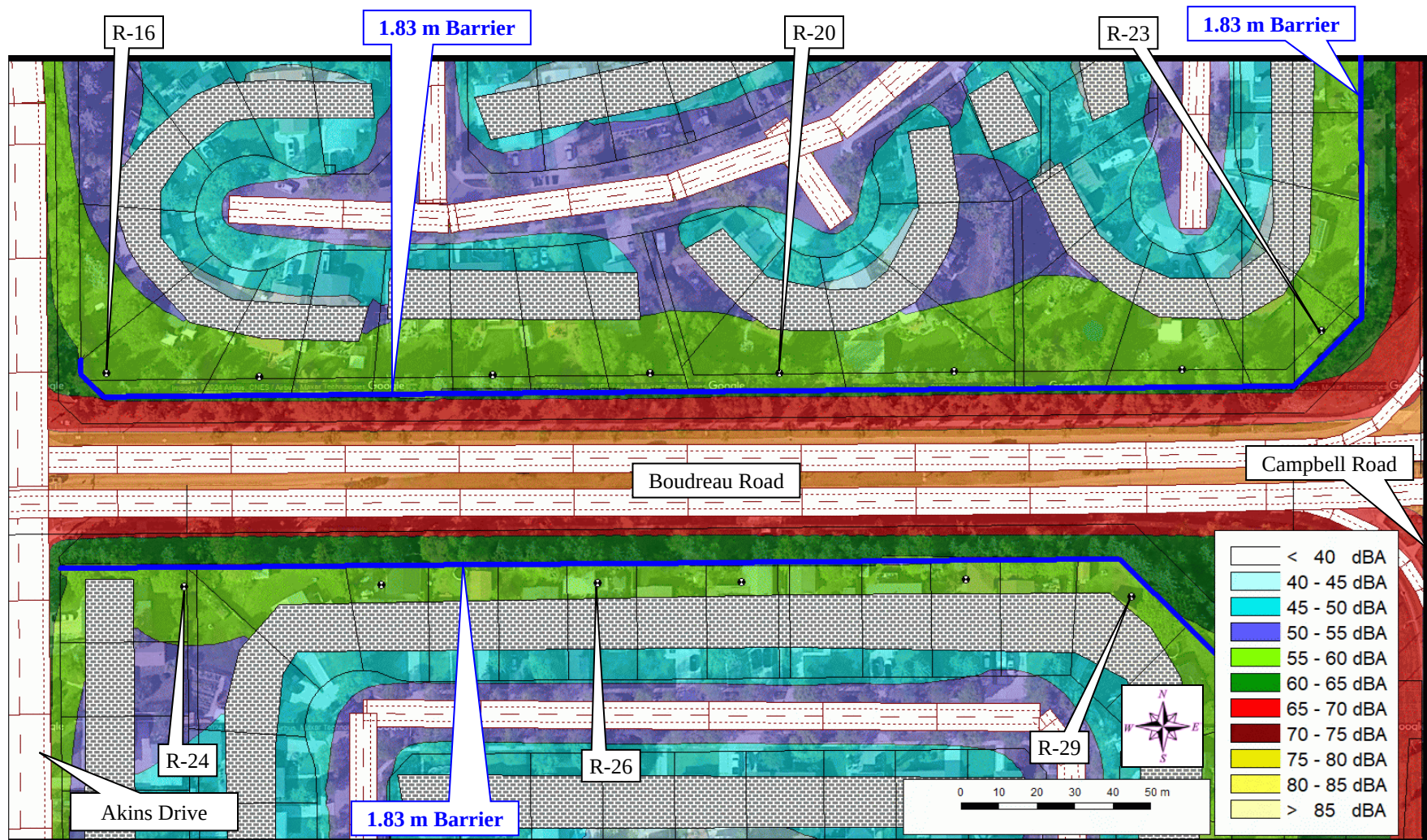
Figure 19. Future Case with Mitigation L_{eq24} Noise Levels (East)
