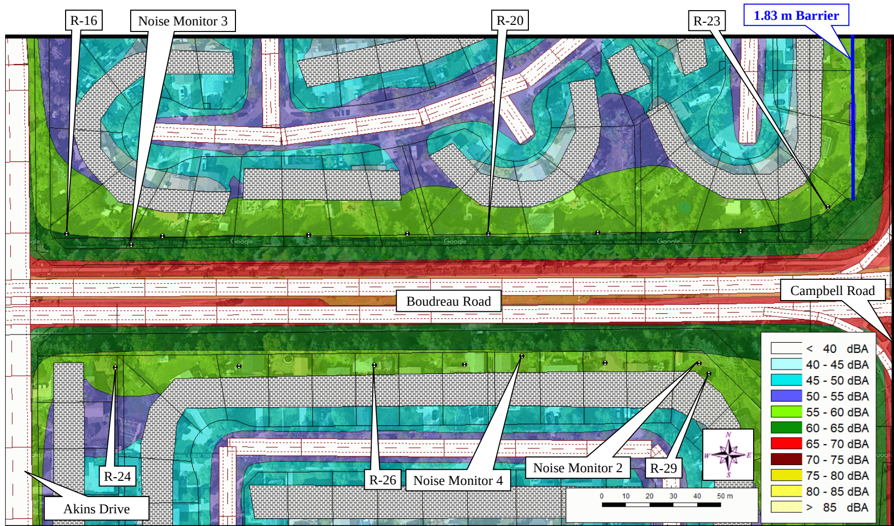
Figure 15. Baseline Case L_{eq24} Noise Levels (East)
