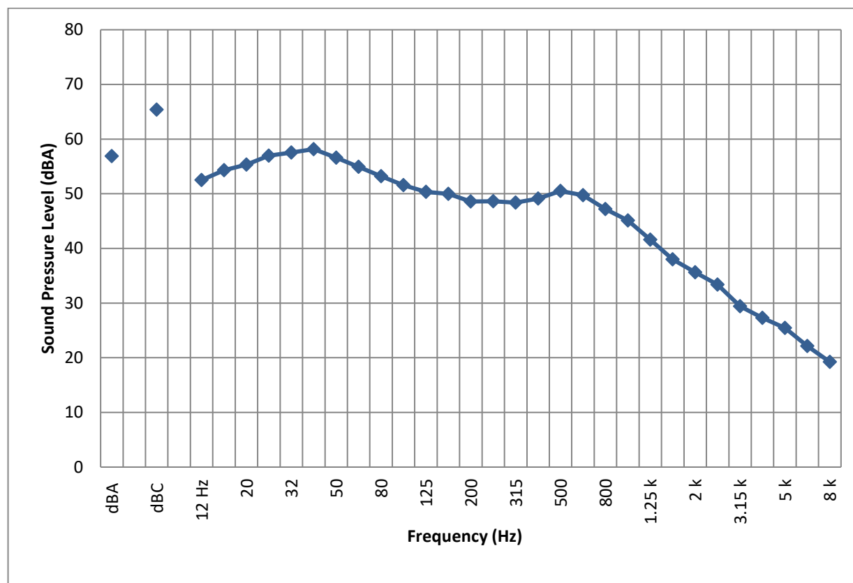
Figure 7. Noise Monitor (60 Aspen Crescent) – 24-Hour 1/3 Octave Band L_{eq} Sound Levels
