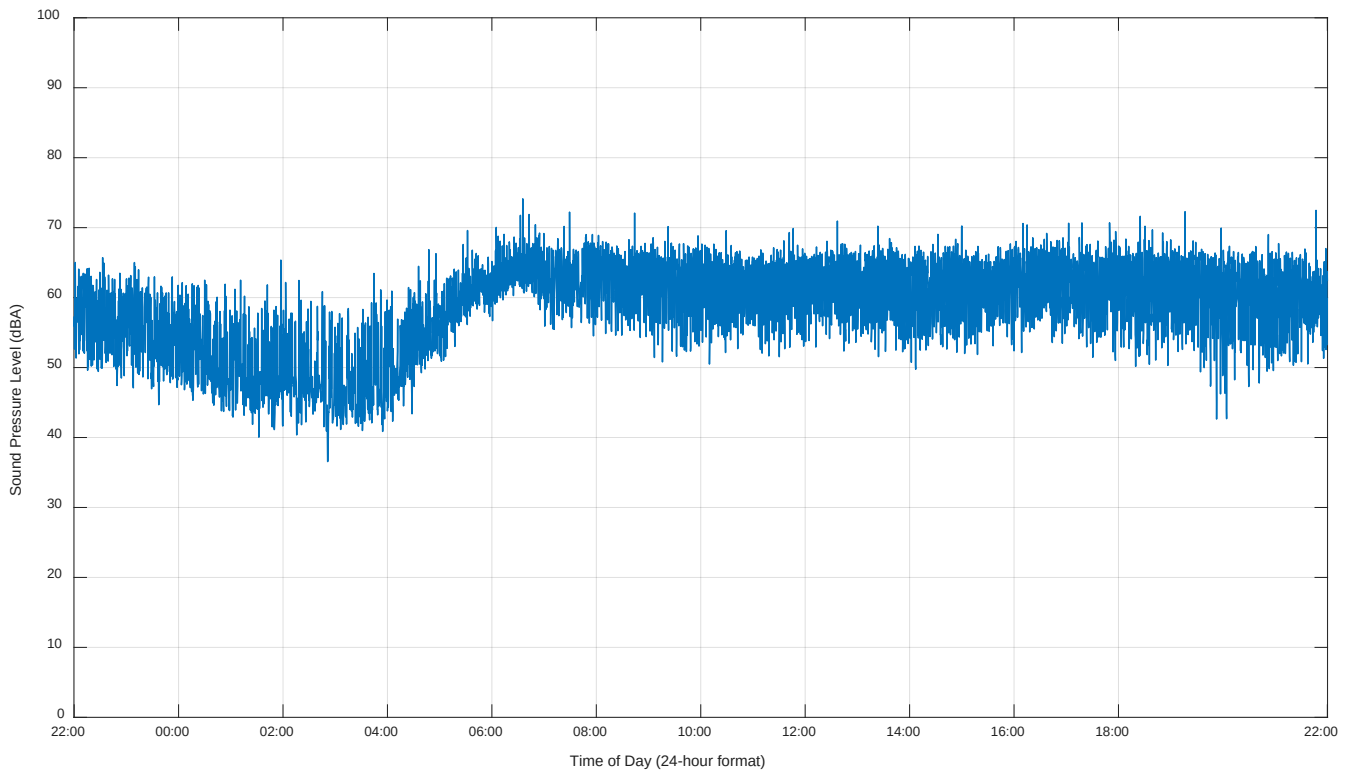
Figure 10. Noise Monitor (15 Patterson Crescent) – 15-Second L_{eq24} Sound Levels
