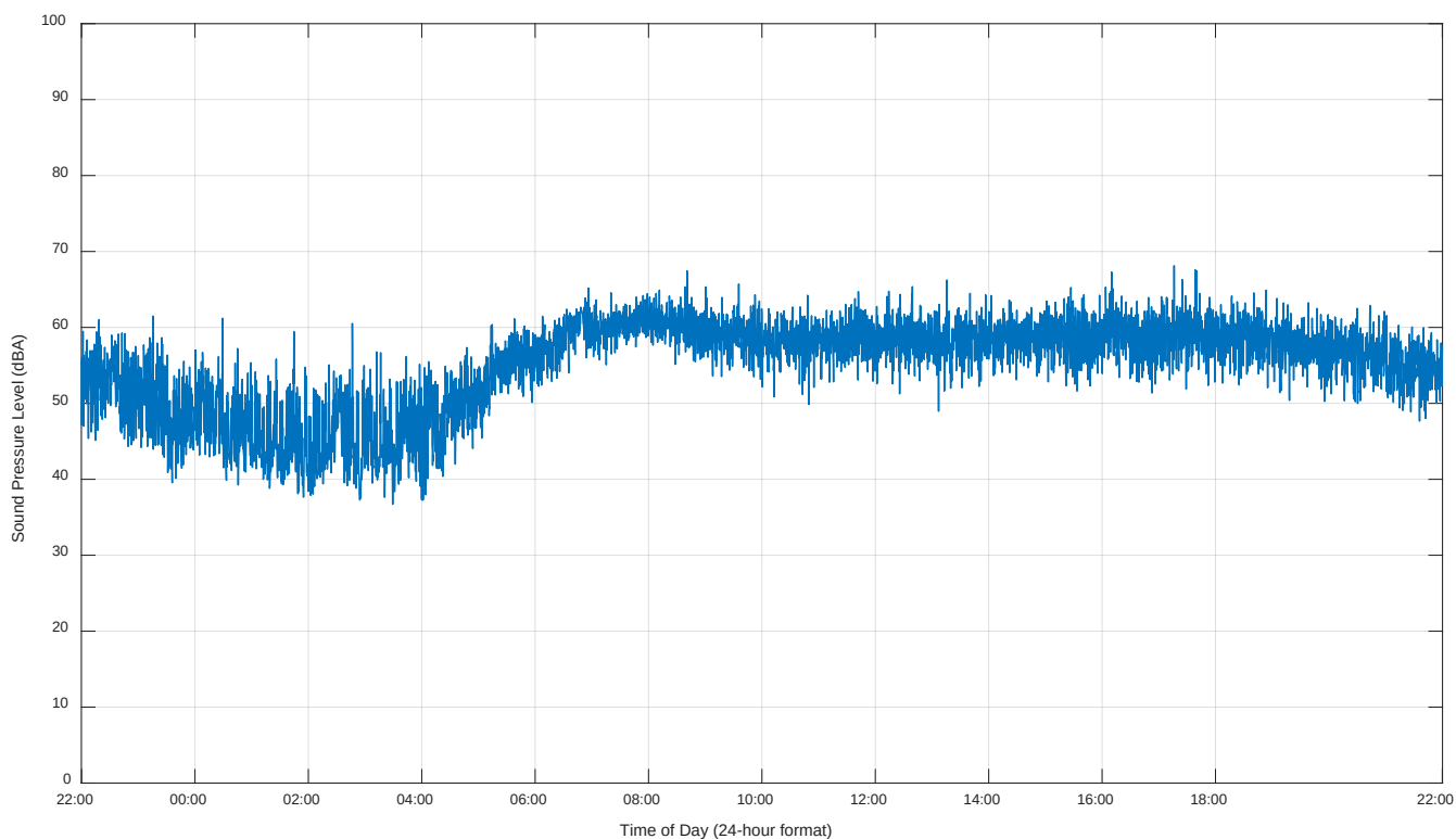
Figure 8. Noise Monitor (44 Andrew Crescent) – 15-Second L_{eq24} Sound Levels
