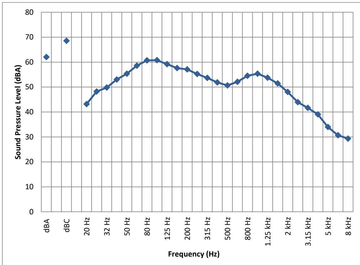
Figure 11. Noise Monitor (15 Patterson Crescent) – 24-Hour 1/3 Octave Band L_{eq} Sound Levels
