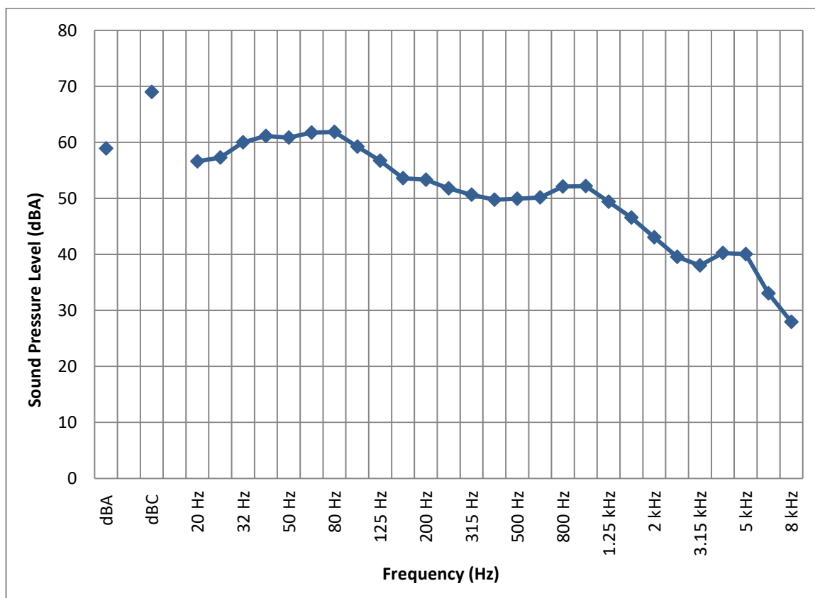
Figure 13. Noise Monitor (52 Andrew Crescent) – 24-Hour 1/3 Octave Band L_{eq} Sound Levels
