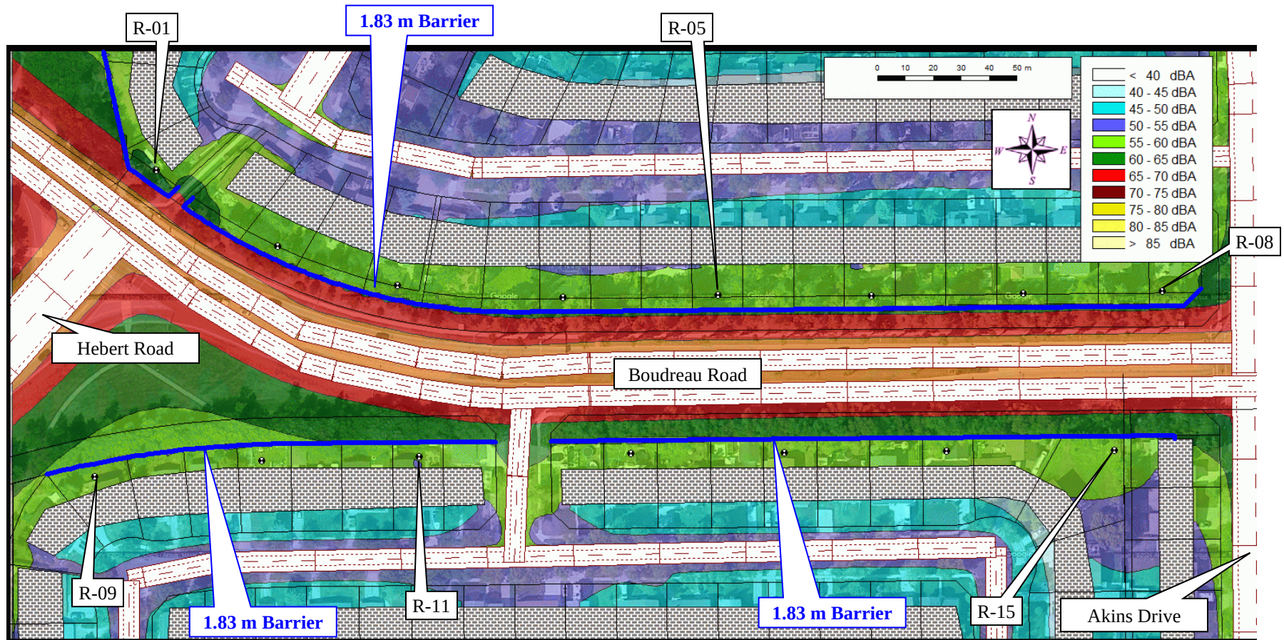
Figure 18. Future Case with Mitigation L_{eq24} Noise Levels (West)
