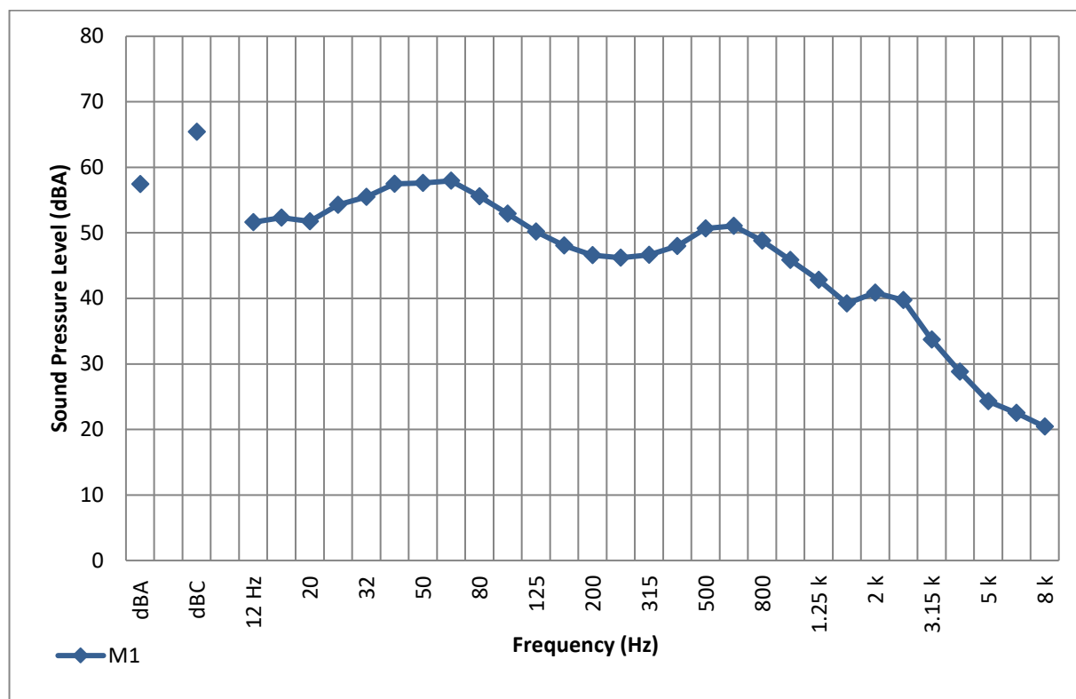
Figure 5. Noise Monitor #1 – 15-Second L_{eq24} Sound Levels
