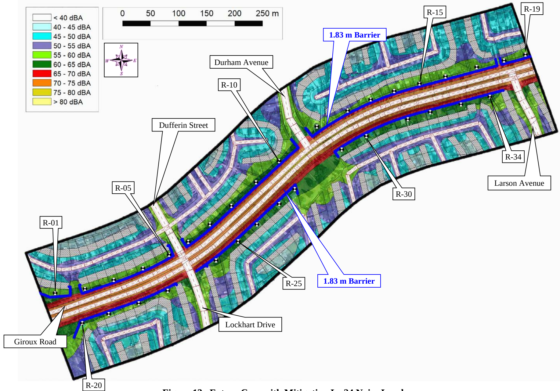
Figure 13. Future Case with Mitigation L_{eq24} Noise Levels
