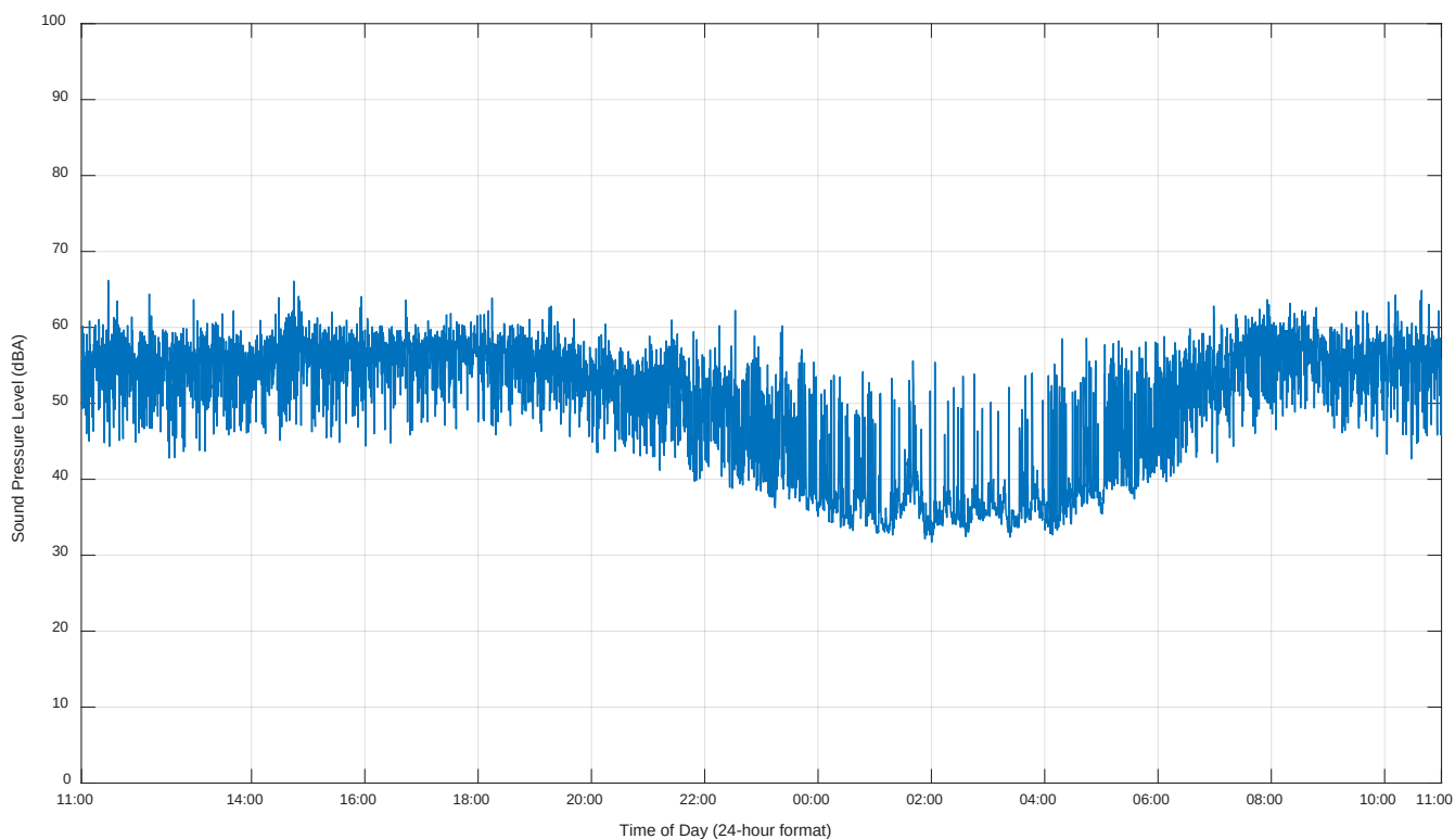
Figure 9. Noise Monitor #3 – 15-Second L_{eq24} Sound Levels
