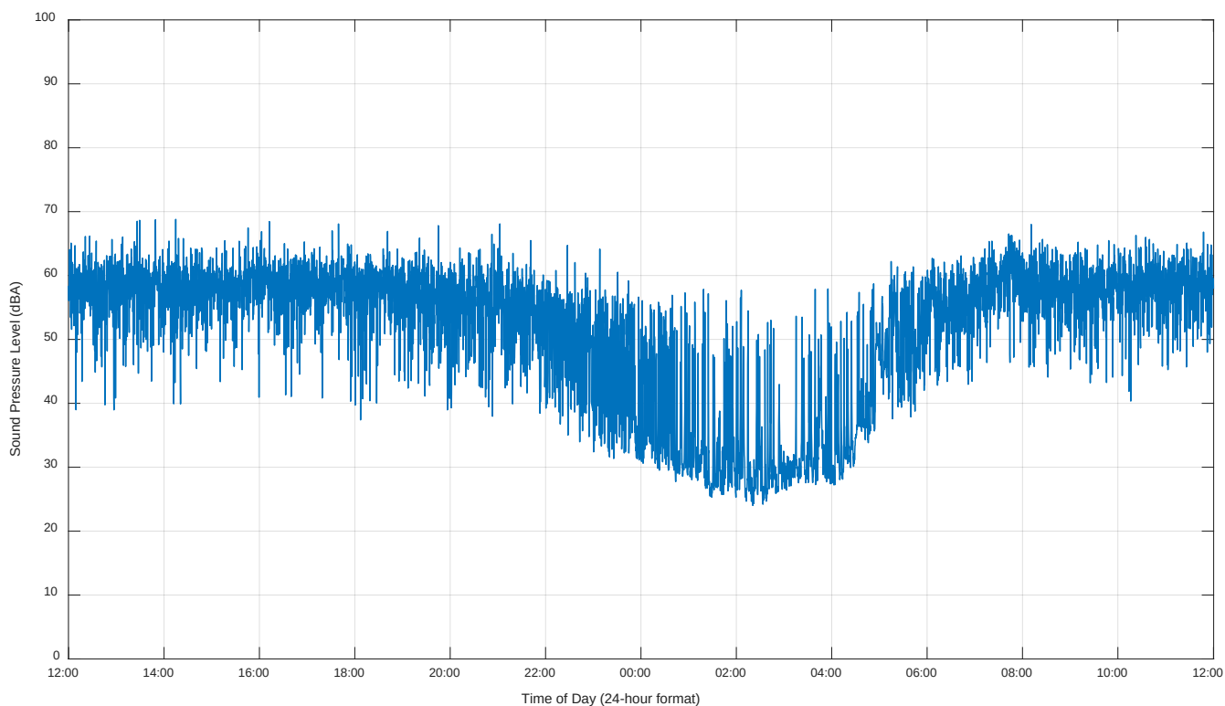
Figure 5. Noise Monitor #1 – 15-Second L_{eq24} Sound Levels
