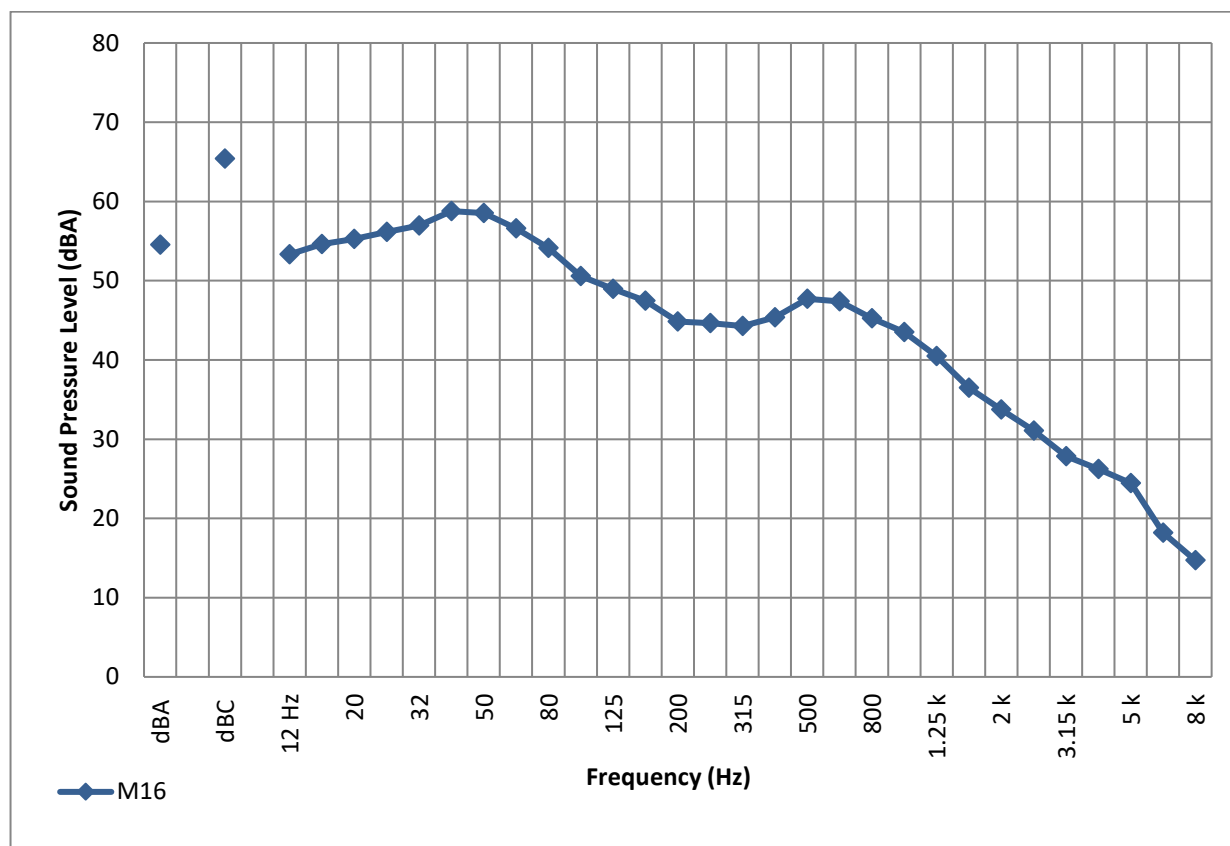
Figure 10. Noise Monitor #3 – 24-Hour 1/3 Octave Band L_{eq} Sound Levels
