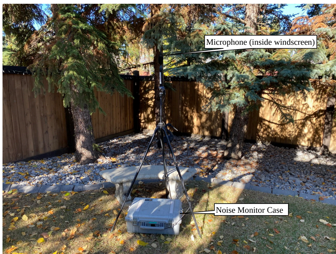
Figure 4. Noise Monitor #3 (38 Lodgepole Crescent)
