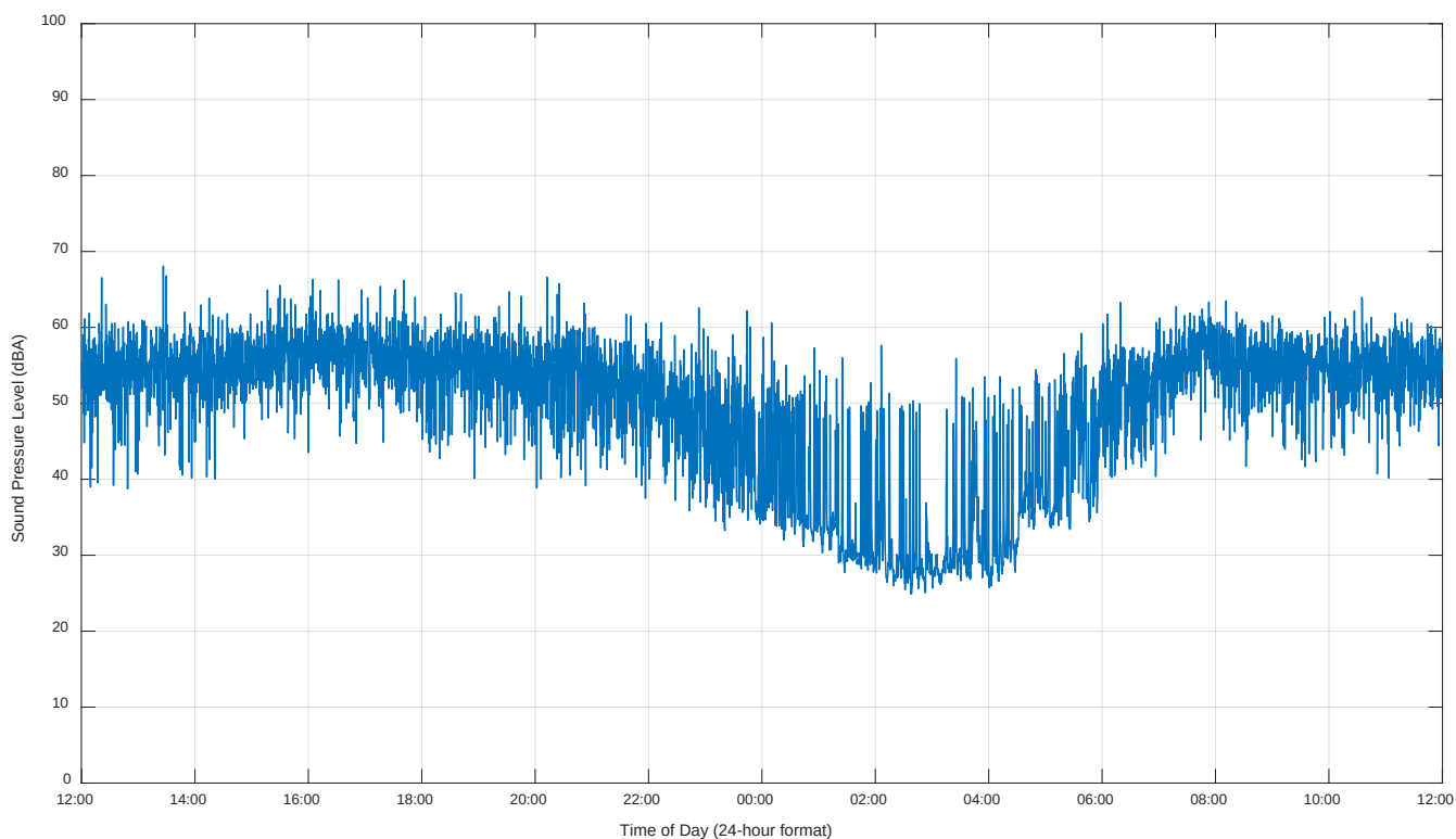
Figure 7. Noise Monitor #2 – 15-Second L_{eq24} Sound Levels
