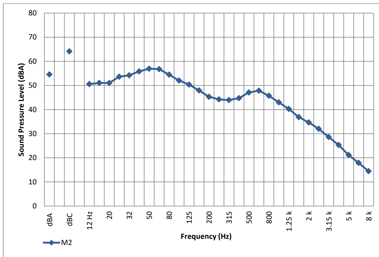
Figure 8. Noise Monitor #2 – 24-Hour 1/3 Octave Band L_{eq} Sound Levels
