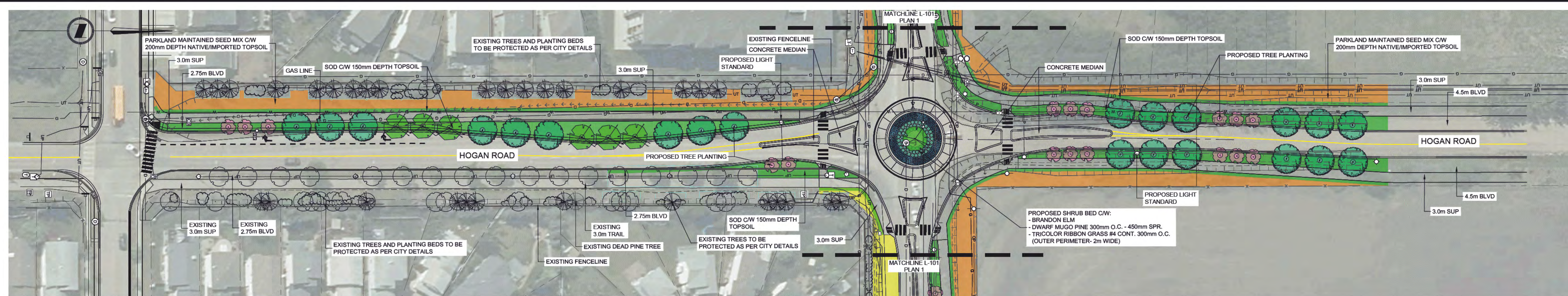
2 HOGAN ROAD - PLAN LAYOUT
